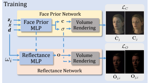
Figure 2: Our Face Prior Network learns to decode latent codes z_j to estimate radiance and volume density for each point in 3D space. Our Reflectance Network learns to synthesize OLAT images of the face.
