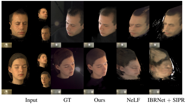
Figure 5: A sample result on the lightstage test set, with groundtruth. Our technique produces novel view synthesis and relightings that clearly outperform NeLF [52] and IBRNet [55] + SIPR [60].
