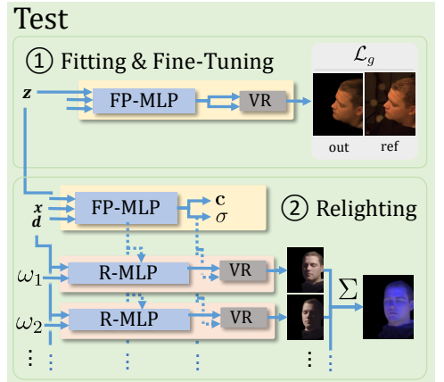
Figure 3: To reconstruct an unseen test face, we optimize latent code \mathbf{z} and fine-tune the Face Prior Network . We can relight the reconstructed face by having the Reflectance Network produce a basis of OLAT images (step 2), that we linearly combine into any desired lighting condition. In this figure, MLP’s with the same label share their weights.
